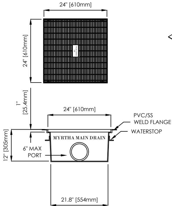
GRATE DETAIL
