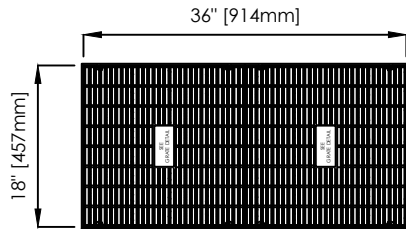
GRATE DETAIL
