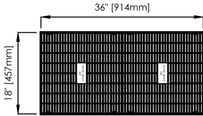
GRATE DETAIL
