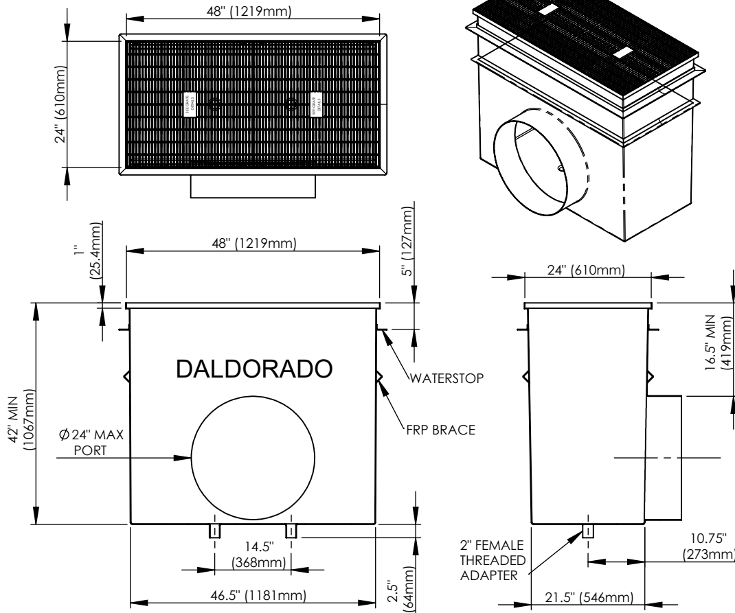
GRATE DETAIL
