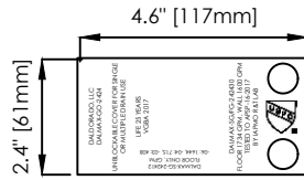
GRATE DETAIL
