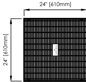
GRATE DETAIL
