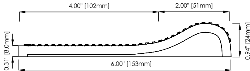
TILE CROSS SECTION
