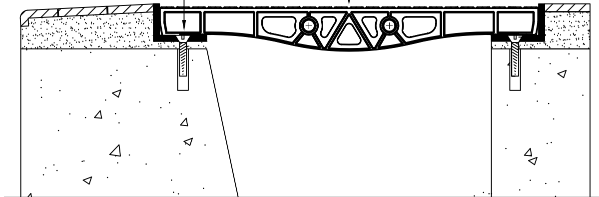
ELEVATION VIEW
