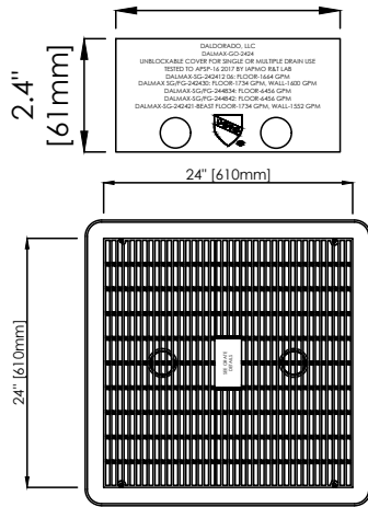
GRATE DETAIL
