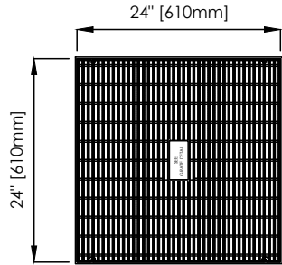
GRATE DETAIL
