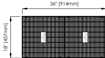
GRATE DETAIL
