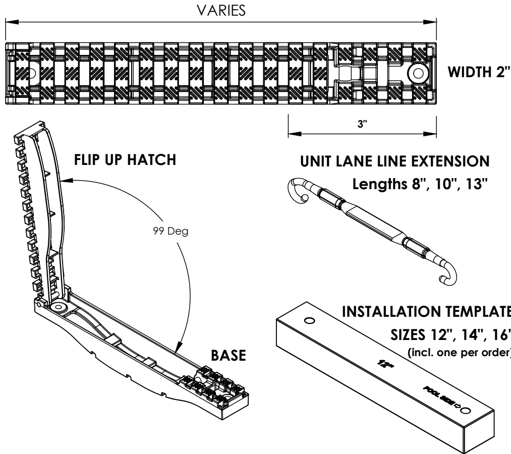
DaIFLEX-LANE-LINE-ANCHOR UNIT PATENT PENDING 63/438,739
