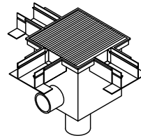
THREE-WAY DDD-DBOX
